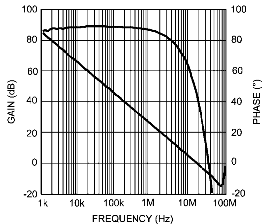
FIGURE 2. LMV796 A_{VOL} vs. Frequency
